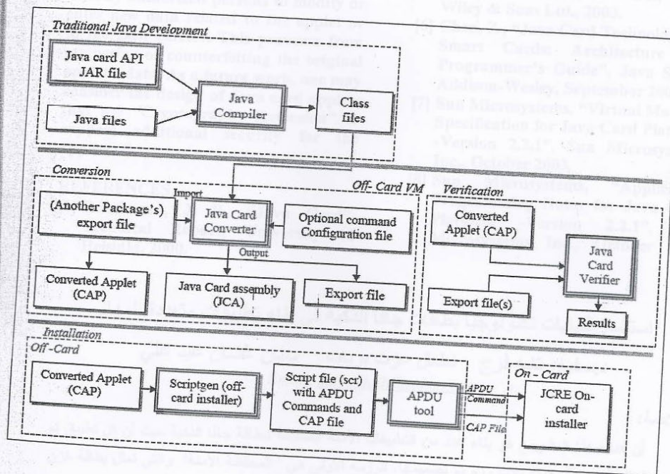
Fig. 5: Java Card applets development steps
