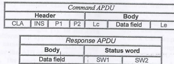
Fig. 3: The command and response APDU formats
