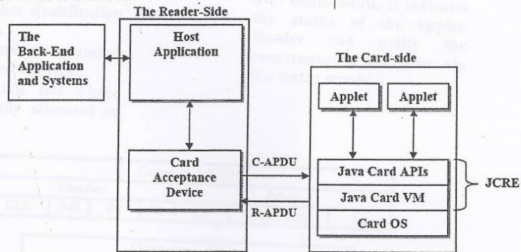
Fig. 2: Elements of Java card applications
