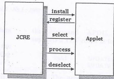
Fig. 4: Interaction between the JCRC and the applet by using the Java Card applet methods
