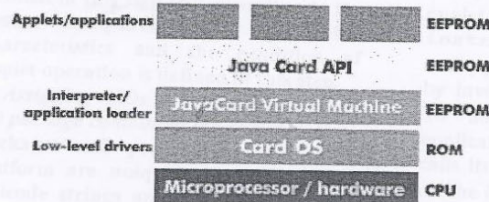
Fig. 1: The basic architecture of Java smart card
